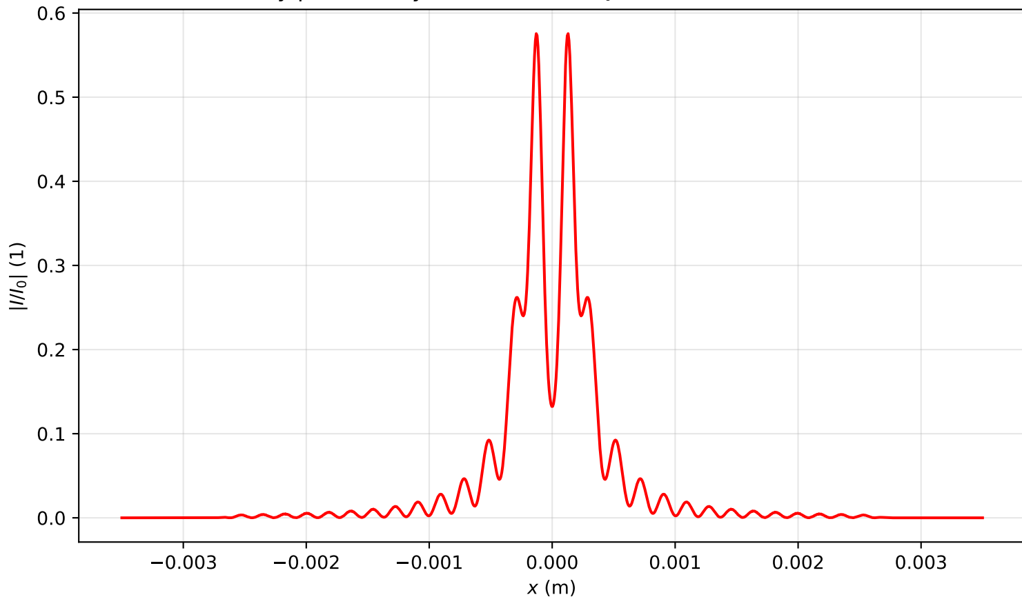
Intensity profile I(x, y = 0, z = 0.159)/I_0 , \text{Pin}=6.0\text{Pcr} , artificial time
